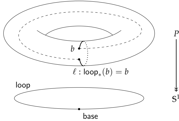
Figure 6.2: The type-theoretic induction principle for \mathbb{S}^1
