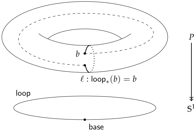
Figure 6.2: The type-theoretic induction principle for \mathbb{S}^1
